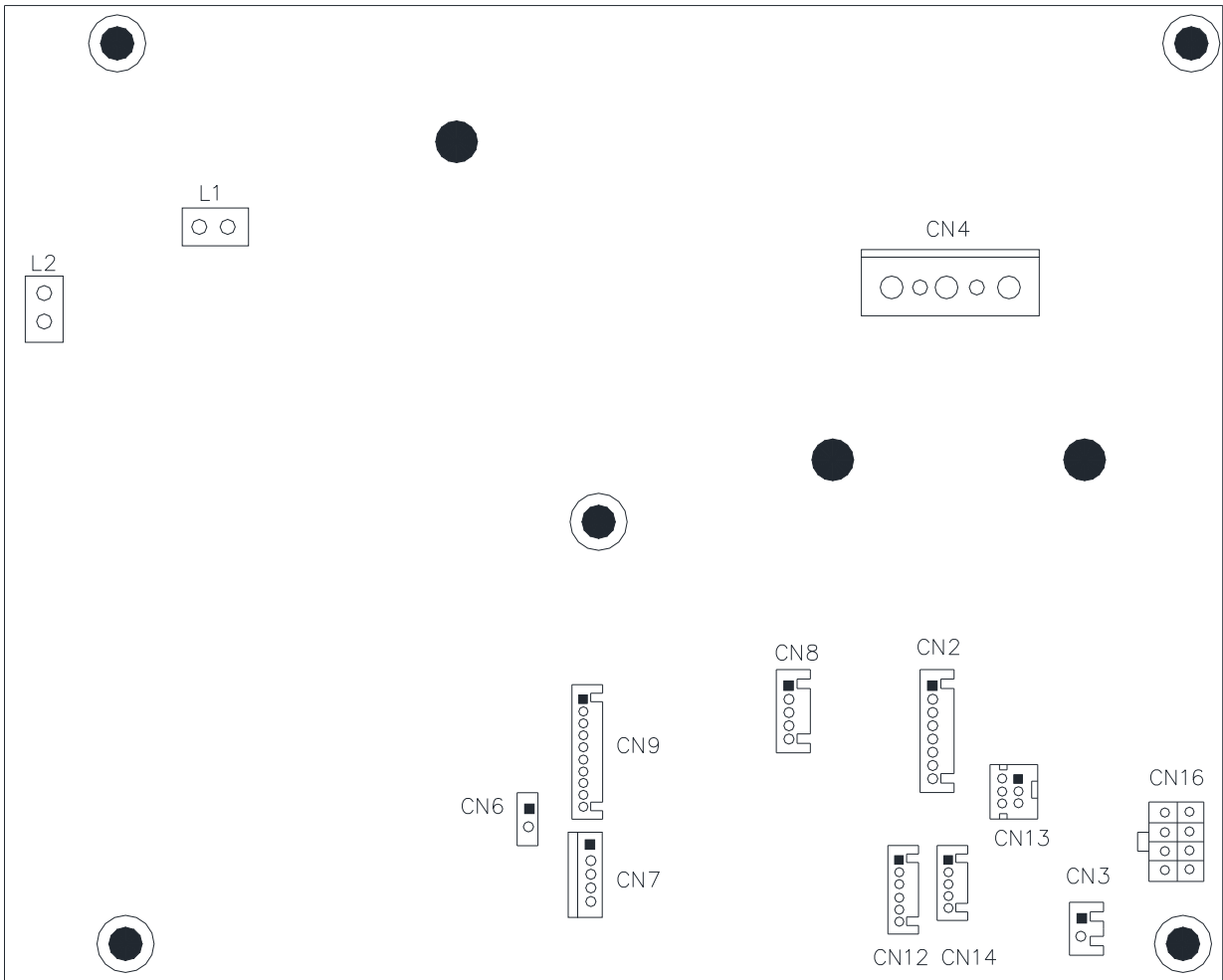
Fig.1B (圖一 B) SV-860E CTL BOARD Connector
